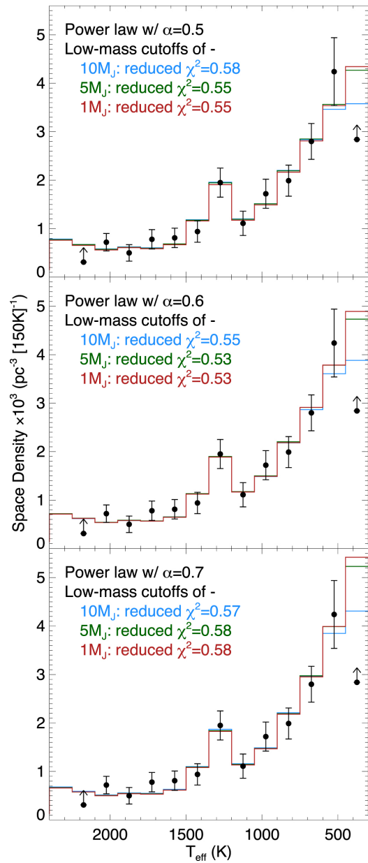
Figure 29. from The Field Substellar Mass Function Based on the Full-sky 20 pc Census of 525 L, T, and Y Dwarfs null 2021 APJS 253 7 doi:10.3847/1538-4365/abd107 https://dx.doi.org/10.3847/1538-4365/abd107 © 2021. The American Astronomical Society. All rights reserved.
