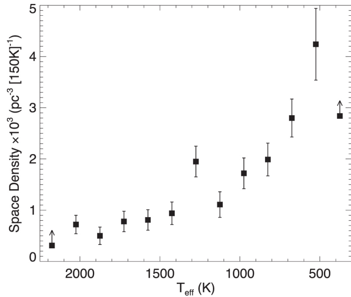
Figure 27. from The Field Substellar Mass Function Based on the Full-sky 20 pc Census of 525 L, T, and Y Dwarfs null 2021 APJS 253 7 doi:10.3847/1538-4365/abd107 https://dx.doi.org/10.3847/1538-4365/abd107
