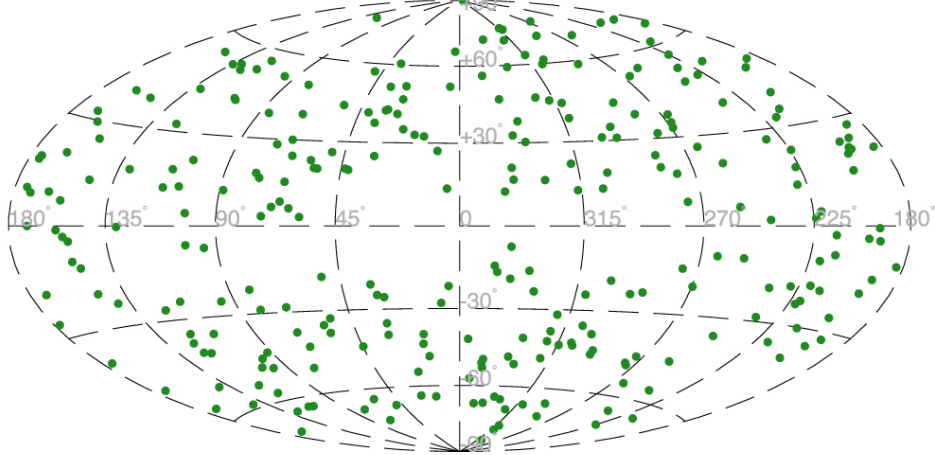
(c) 20-pc census - T Dwarfs Only
