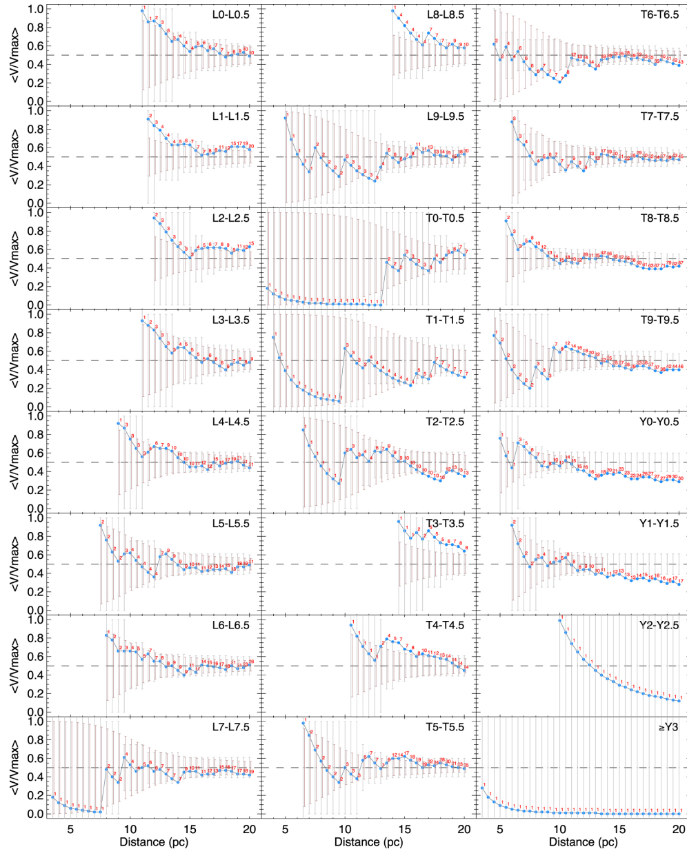
Figure 24. from The Field Substellar Mass Function Based on the Full-sky 20 pc Census of 525 L, T, and Y Dwarfs null 2021 APJS 253 7 doi:10.3847/1538-4365/abd107 https://dx.doi.org/10.3847/1538-4365/abd107
