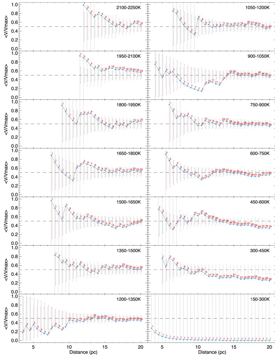
Figure 23. from The Field Substellar Mass Function Based on the Full-sky 20 pc Census of 525 L, T, and Y Dwarfs null 2021 APJS 253 7 doi:10.3847/1538-4365/abd107 https://dx.doi.org/10.3847/1538-4365/abd107
