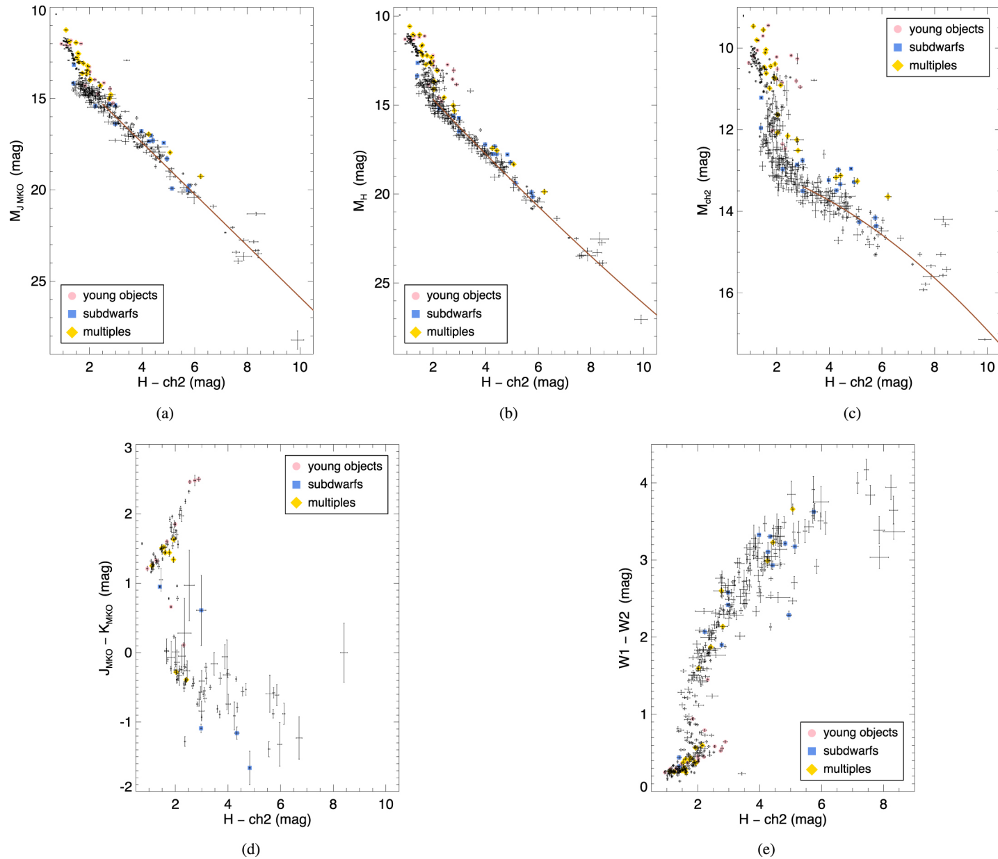
Figure 21. from The Field Substellar Mass Function Based on the Full-sky 20 pc Census of 525 L, T, and Y Dwarfs null 2021 APJS 253 7 doi:10.3847/1538-4365/abd107 https://dx.doi.org/10.3847/1538-4365/abd107
