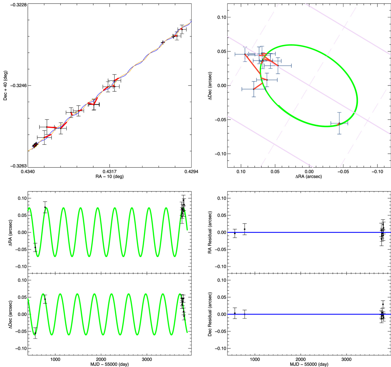
Figure 2. from The Field Substellar Mass Function Based on the Full-sky 20 pc Census of 525 L, T, and Y Dwarfs null 2021 APJS 253 7 doi:10.3847/1538-4365/abd107 https://dx.doi.org/10.3847/1538-4365/abd107 © 2021. The American Astronomical Society. All rights reserved.
