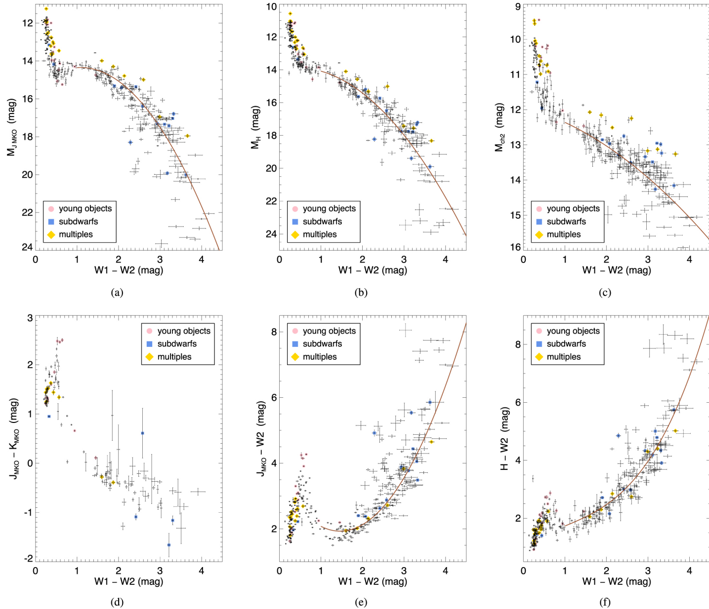
Figure 19. from The Field Substellar Mass Function Based on the Full-sky 20 pc Census of 525 L, T, and Y Dwarfs null 2021 APJS 253 7 doi:10.3847/1538-4365/abd107 https://dx.doi.org/10.3847/1538-4365/abd107
