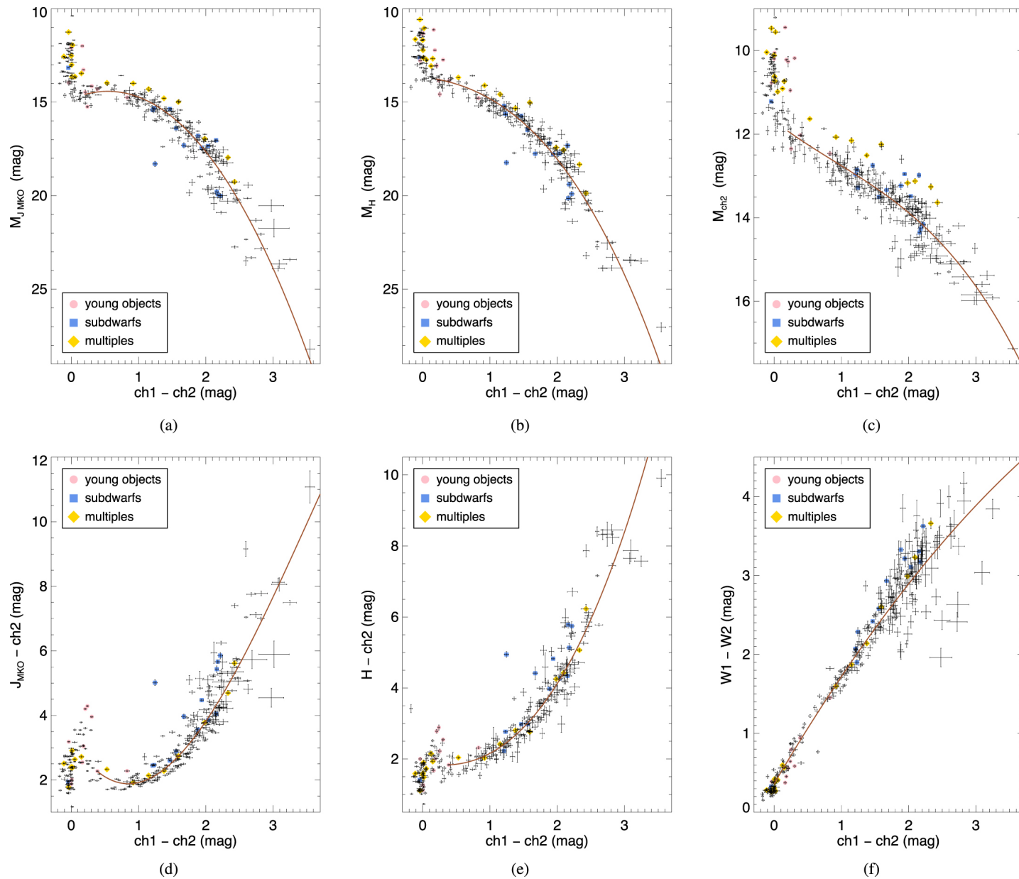
Figure 18. from The Field Substellar Mass Function Based on the Full-sky 20 pc Census of 525 L, T, and Y Dwarfs null 2021 APJS 253 7 doi:10.3847/1538-4365/abd107 https://dx.doi.org/10.3847/1538-4365/abd107
