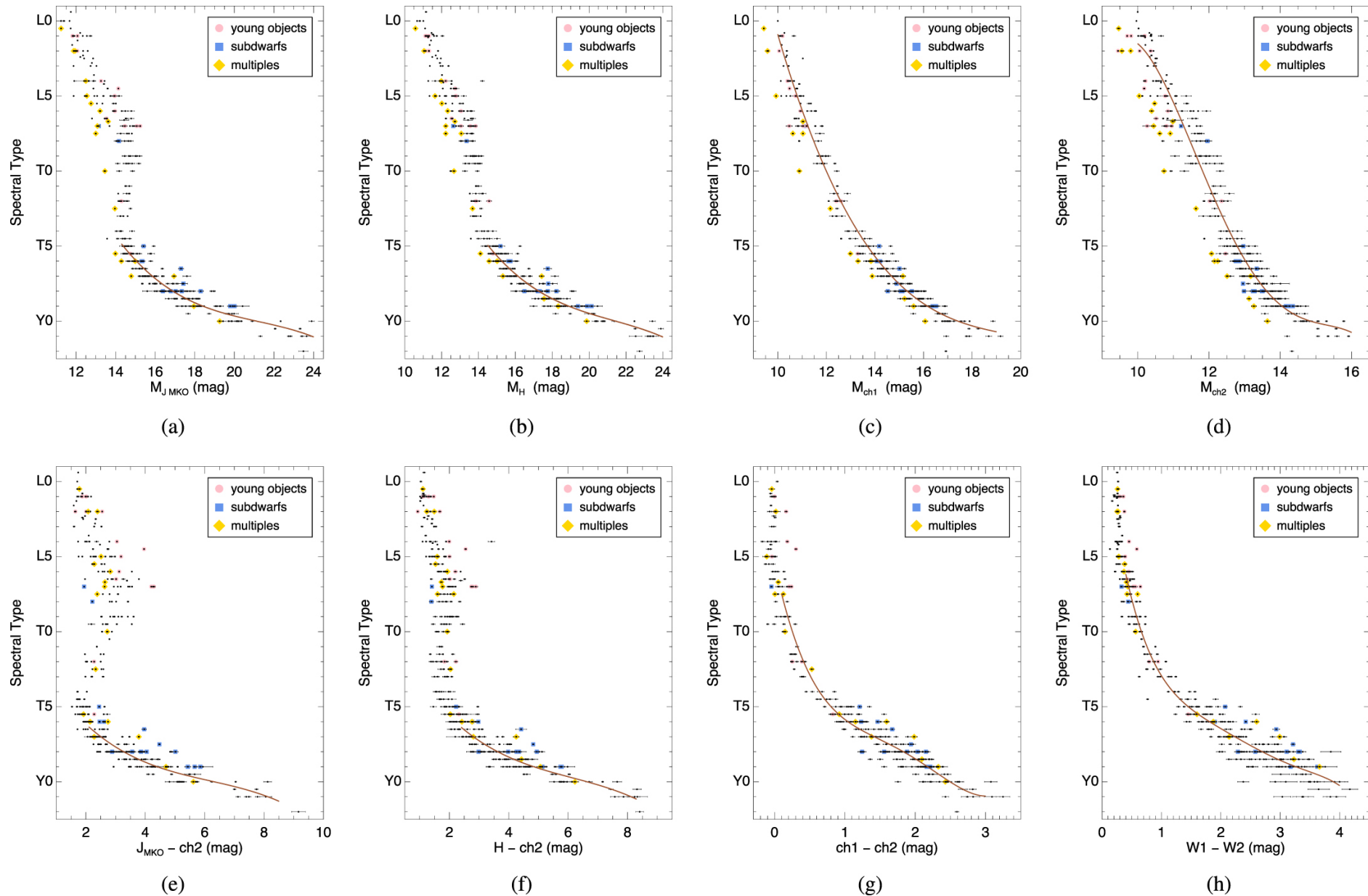
Figure 17. from The Field Substellar Mass Function Based on the Full-sky 20 pc Census of 525 L, T, and Y Dwarfs null 2021 APJS 253 7 doi:10.3847/1538-4365/abd107 https://dx.doi.org/10.3847/1538-4365/abd107
