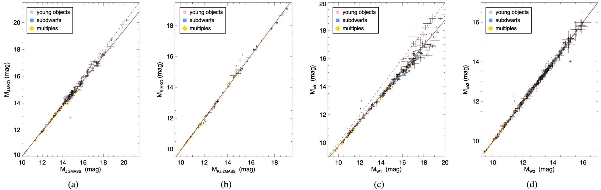
Figure 14. from The Field Substellar Mass Function Based on the Full-sky 20 pc Census of 525 L, T, and Y Dwarfs null 2021 APJS 253 7 doi:10.3847/1538-4365/abd107 https://dx.doi.org/10.3847/1538-4365/abd107 © 2021. The American Astronomical Society. All rights reserved.
