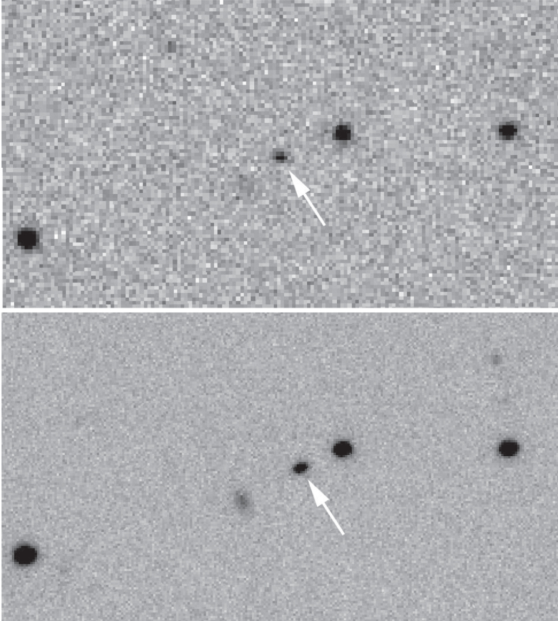
Figure 12. from The Field Substellar Mass Function Based on the Full-sky 20 pc Census of 525 L, T, and Y Dwarfs null 2021 APJS 253 7 doi:10.3847/1538-4365/abd107 https://dx.doi.org/10.3847/1538-4365/abd107 © 2021. The American Astronomical Society. All rights reserved.
