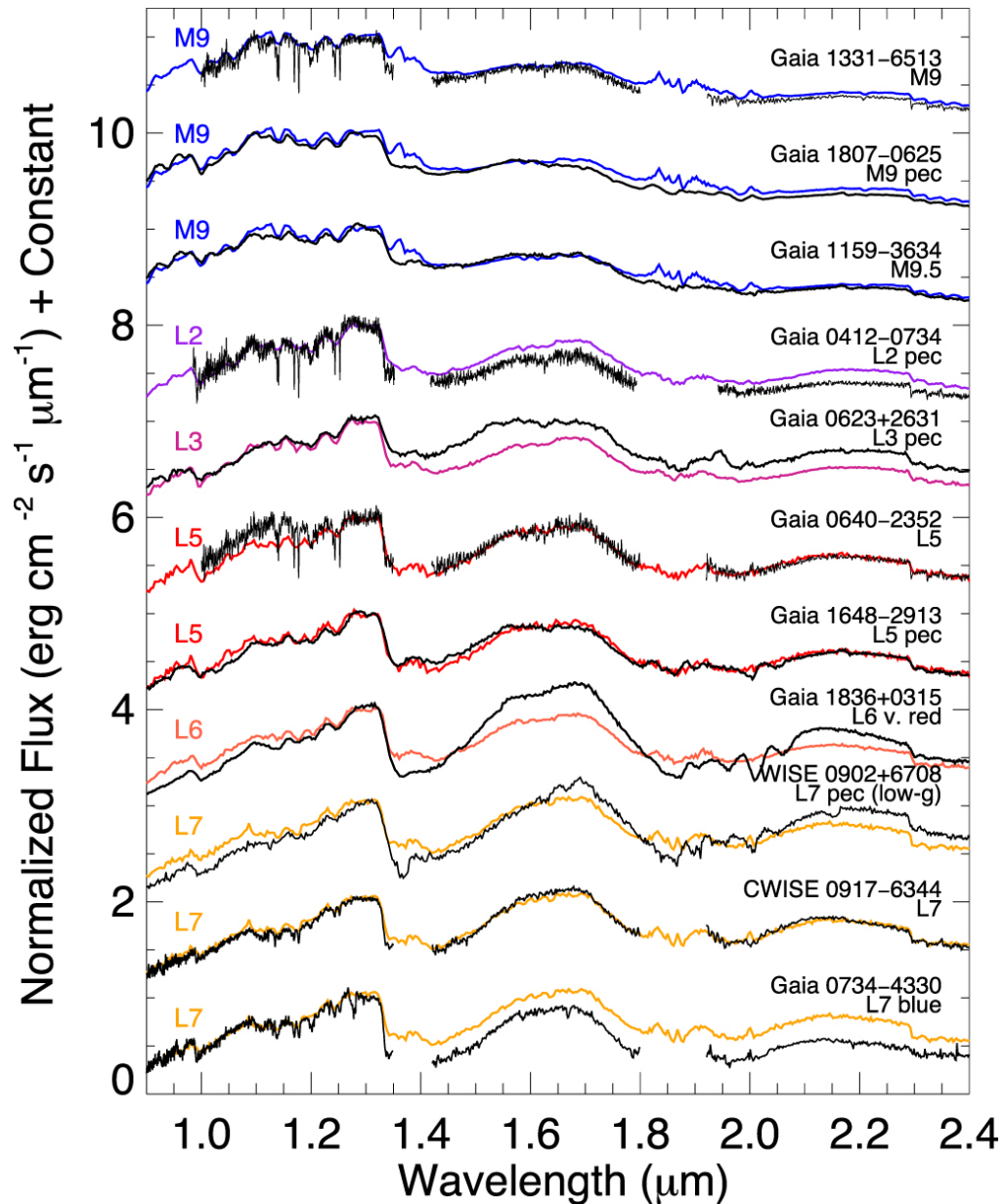
Figure 10. from The Field Substellar Mass Function Based on the Full-sky 20 pc Census of 525 L, T, and Y Dwarfs null 2021 APJS 253 7 doi:10.3847/1538-4365/abd107 https://dx.doi.org/10.3847/1538-4365/abd107 © 2021. The American Astronomical Society. All rights reserved.
