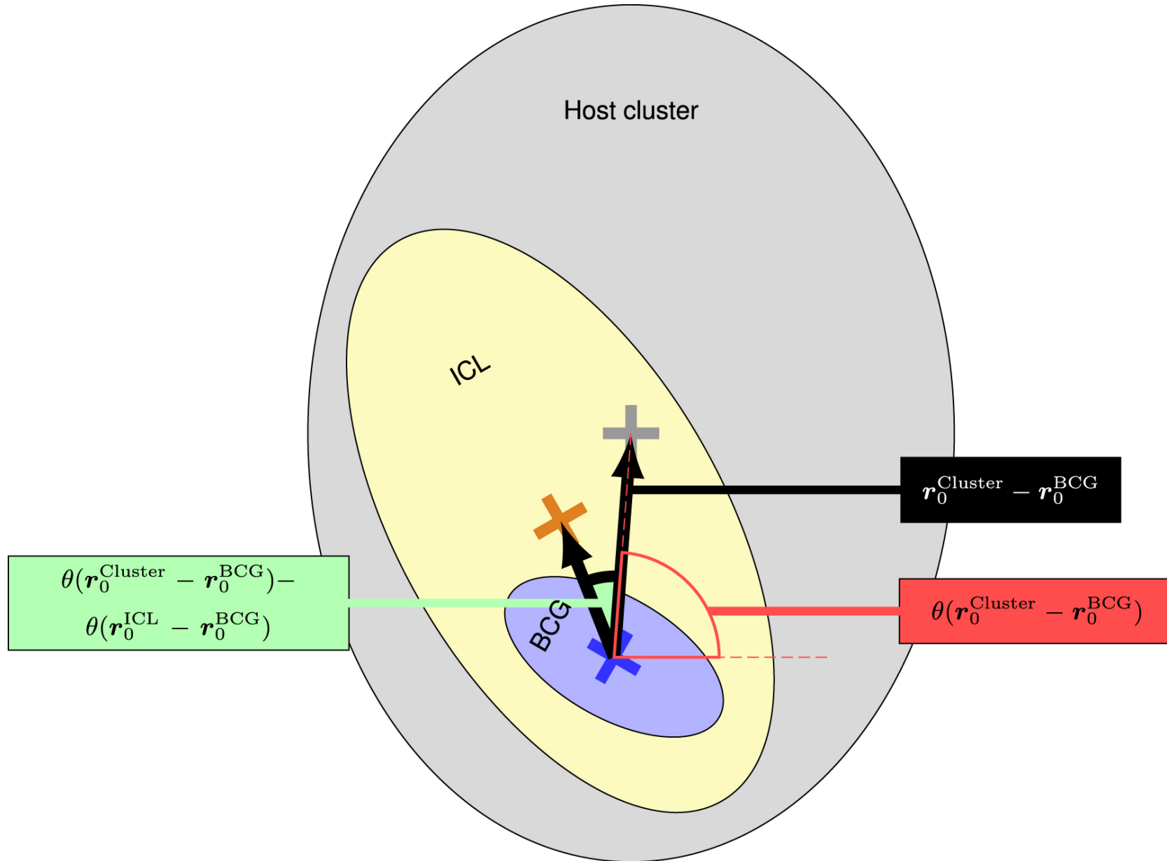
Figure 3. from Photometric Dissection of Intracluster Light and Its Correlations with Host Cluster Properties null 2021 APJS 252 27 doi:10.3847/1538-4365/abcda6 https://dx.doi.org/10.3847/1538-4365/abcda6 © 2021. The American Astronomical Society. All rights reserved.
