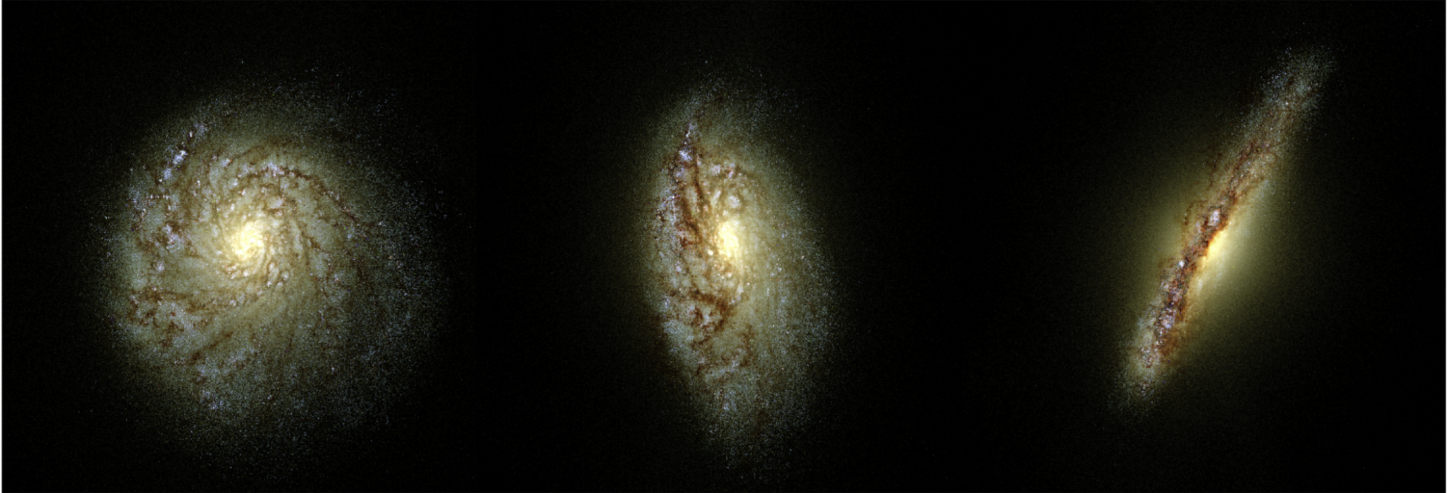
Figure 10. from POWDERDAY: Dust Radiative Transfer for Galaxy Simulations null 2021 APJS 252 12 doi:10.3847/1538-4365/abc487 https://dx.doi.org/10.3847/1538-4365/abc487 © 2021. The American Astronomical Society. All rights reserved.
