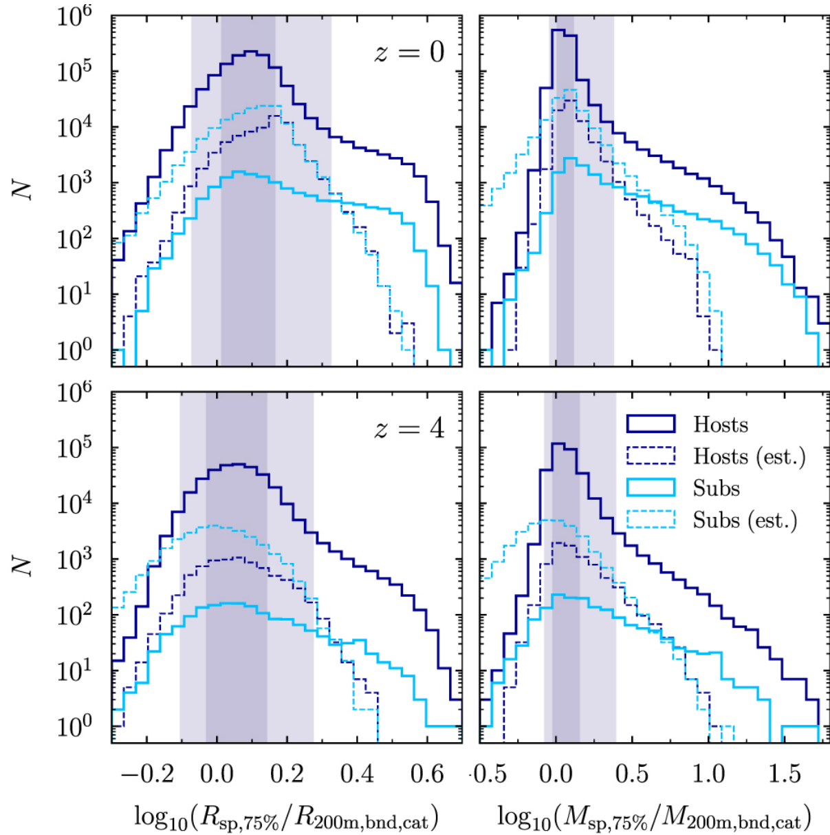
Figure 9. from The Splashback Radius of Halos from Particle Dynamics. III. Halo Catalogs, Merger Trees, and Host–Subhalo Relations null 2020 APJS 251 17 doi:10.3847/1538-4365/abfb51 https://dx.doi.org/10.3847/1538-4365/abfb51
