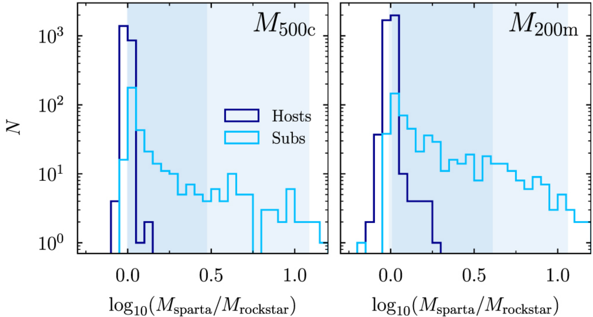
Figure 8. from The Splashback Radius of Halos from Particle Dynamics. III. Halo Catalogs, Merger Trees, and Host–Subhalo Relations null 2020 APJS 251 17 doi:10.3847/1538-4365/abbf51 https://dx.doi.org/10.3847/1538-4365/abbf51 © 2020. The American Astronomical Society. All rights reserved.
