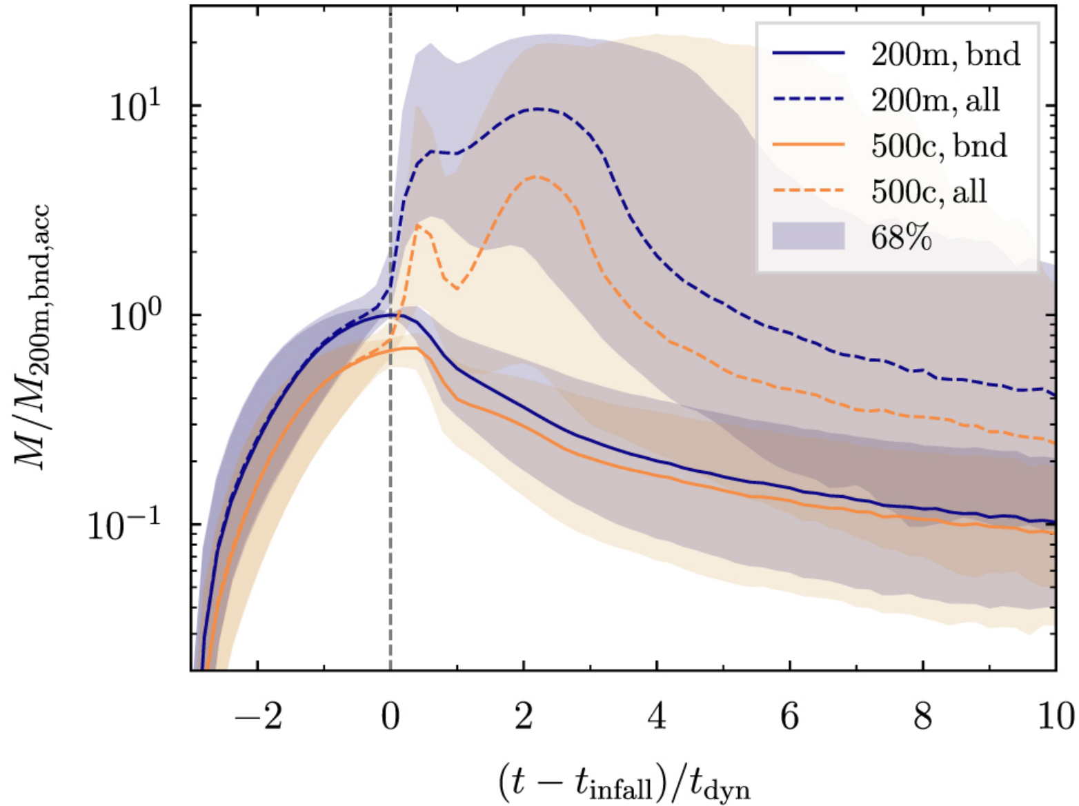
Figure 7. from The Splashback Radius of Halos from Particle Dynamics. III. Halo Catalogs, Merger Trees, and Host–Subhalo Relations null 2020 APJS 251 17 doi:10.3847/1538-4365/abbf51 https://dx.doi.org/10.3847/1538-4365/abbf51 © 2020. The American Astronomical Society. All rights reserved.
