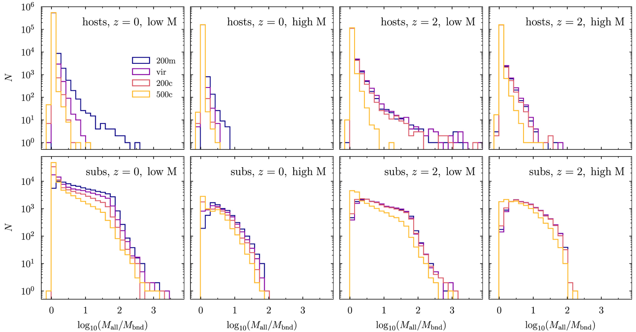
Figure 6. from The Splashback Radius of Halos from Particle Dynamics. III. Halo Catalogs, Merger Trees, and Host–Subhalo Relations null 2020 APJS 251 17 doi:10.3847/1538-4365/abfb51 https://dx.doi.org/10.3847/1538-4365/abfb51 © 2020. The American Astronomical Society. All rights reserved.
