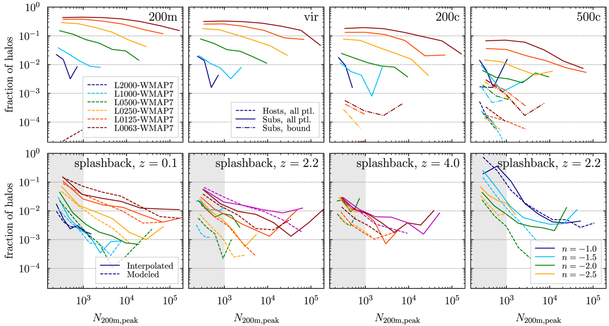
Figure 5. from The Splashback Radius of Halos from Particle Dynamics. III. Halo Catalogs, Merger Trees, and Host–Subhalo Relations null 2020 APJS 251 17 doi:10.3847/1538-4365/abf51 https://dx.doi.org/10.3847/1538-4365/abf51 © 2020. The American Astronomical Society. All rights reserved.
