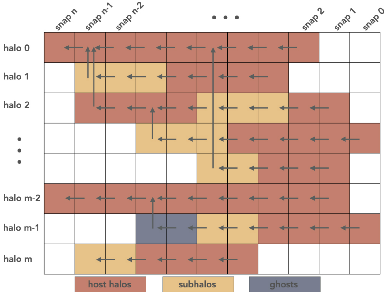
Figure 4. from The Splashback Radius of Halos from Particle Dynamics. III. Halo Catalogs, Merger Trees, and Host–Subhalo Relations null 2020 APJS 251 17 doi:10.3847/1538-4365/abbbf51 https://dx.doi.org/10.3847/1538-4365/abbbf51 © 2020. The American Astronomical Society. All rights reserved.
