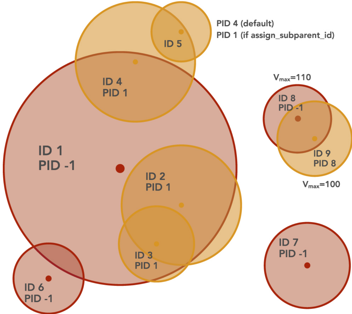
Figure 3. from The Splashback Radius of Halos from Particle Dynamics. III. Halo Catalogs, Merger Trees, and Host–Subhalo Relations null 2020 APJS 251 17 doi:10.3847/1538-4365/abbf51 https://dx.doi.org/10.3847/1538-4365/abbf51 © 2020. The American Astronomical Society. All rights reserved.
