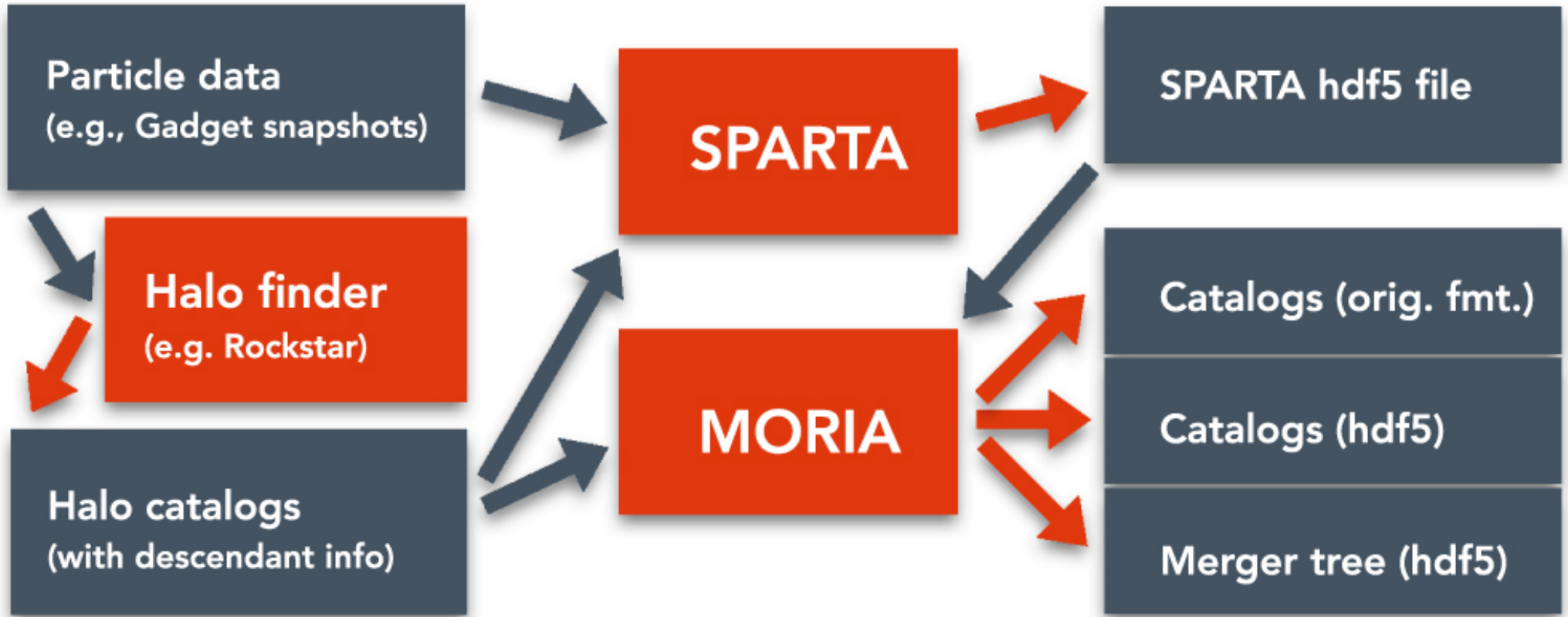
Figure 2. from The Splashback Radius of Halos from Particle Dynamics. III. Halo Catalogs, Merger Trees, and Host–Subhalo Relations null 2020 APJS 251 17 doi:10.3847/1538-4365/abfb51 https://dx.doi.org/10.3847/1538-4365/abfb51 © 2020. The American Astronomical Society. All rights reserved.
