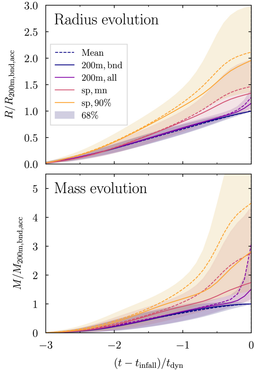
Figure 10. from The Splashback Radius of Halos from Particle Dynamics. III. Halo Catalogs, Merger Trees, and Host–Subhalo Relations null 2020 APJS 251 17 doi:10.3847/1538-4365/abf51 https://dx.doi.org/10.3847/1538-4365/abf51
