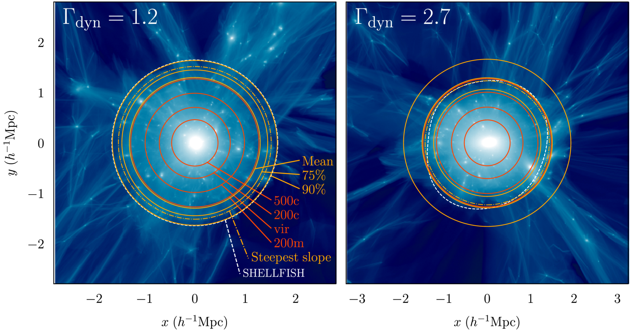
Figure 1. from The Splashback Radius of Halos from Particle Dynamics. III. Halo Catalogs, Merger Trees, and Host–Subhalo Relations null 2020 APJS 251 17 doi:10.3847/1538-4365/abbf51 https://dx.doi.org/10.3847/1538-4365/abbf51 © 2020. The American Astronomical Society. All rights reserved.
