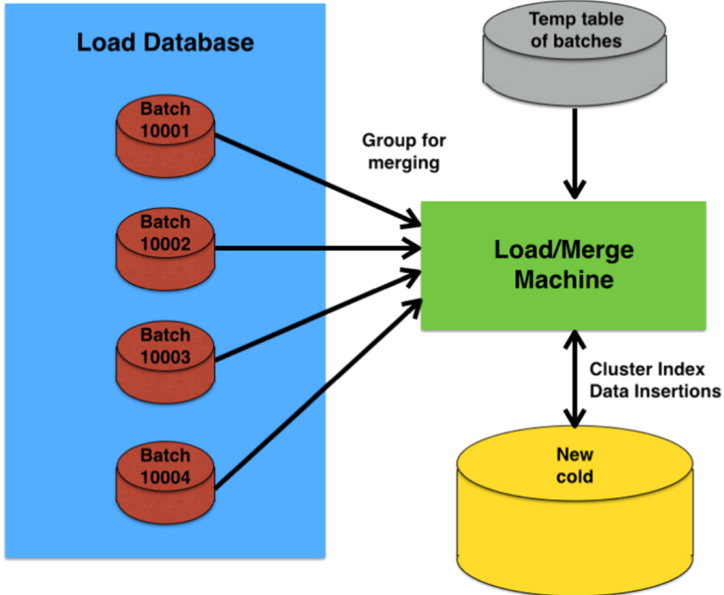
Figure 7. from The Pan-STARRS1 Database and Data Products null 2020 APJS 251 7 doi:10.3847/1538-4365/abb82d https://dx.doi.org/10.3847/1538-4365/abb82d © 2020. The American Astronomical Society. All rights reserved.
