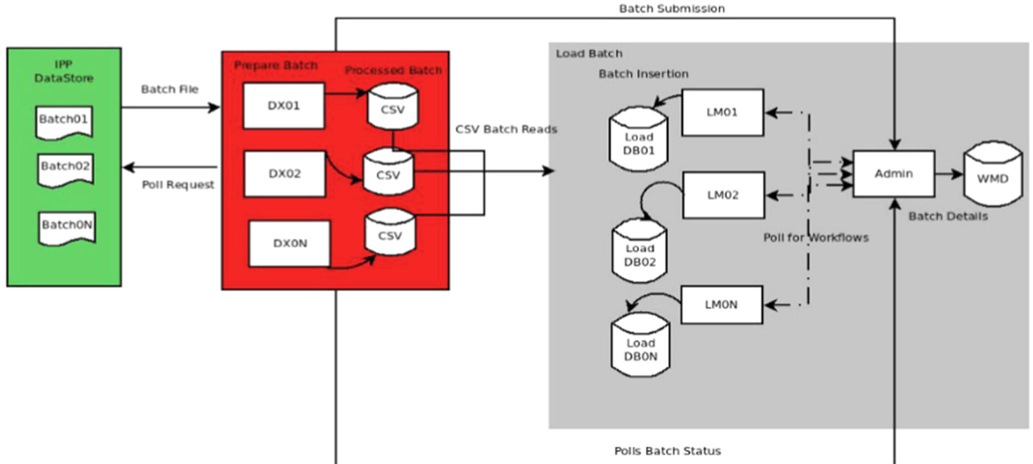
Figure 6. from The Pan-STARRS1 Database and Data Products null 2020 APJS 251 7 doi:10.3847/1538-4365/abb82d https://dx.doi.org/10.3847/1538-4365/abb82d © 2020. The American Astronomical Society. All rights reserved.
