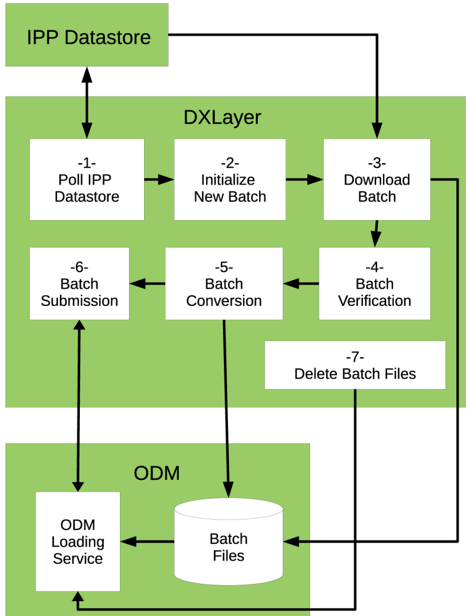
Figure 5. from The Pan-STARRS1 Database and Data Products null 2020 APJS 251 7 doi:10.3847/1538-4365/abb82d https://dx.doi.org/10.3847/1538-4365/abb82d © 2020. The American Astronomical Society. All rights reserved.
