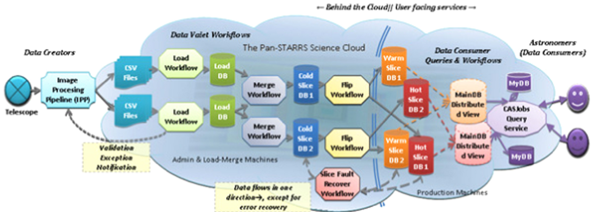
Figure 3. from The Pan-STARRS1 Database and Data Products null 2020 APJS 251 7 doi:10.3847/1538-4365/abb82d https://dx.doi.org/10.3847/1538-4365/abb82d © 2020. The American Astronomical Society. All rights reserved.
