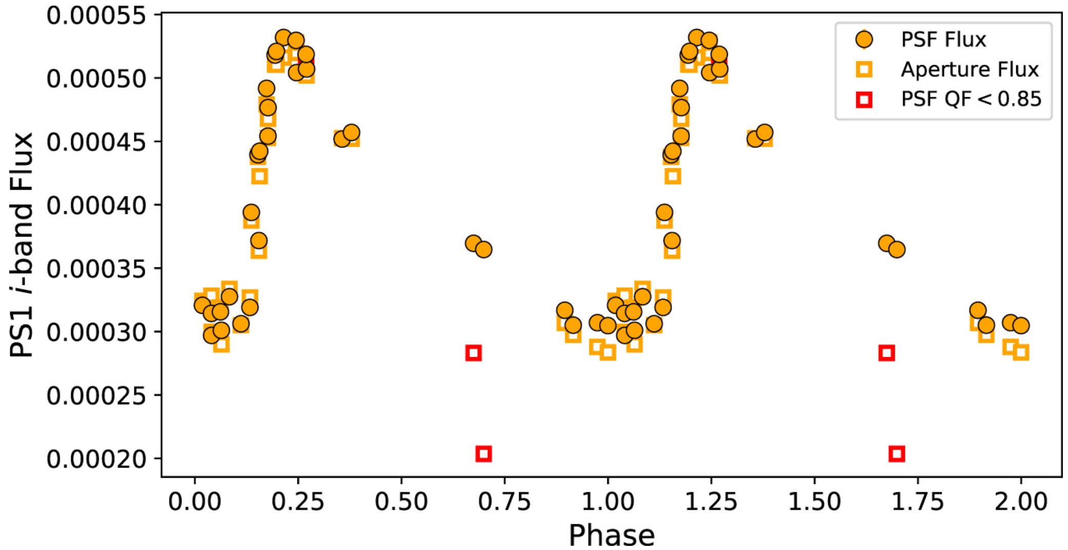
Figure 11. from The Pan-STARRS1 Database and Data Products null 2020 APJS 251 7 doi:10.3847/1538-4365/abb82d https://dx.doi.org/10.3847/1538-4365/abb82d © 2020. The American Astronomical Society. All rights reserved.
