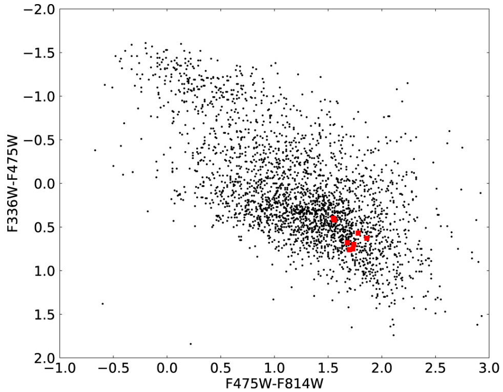
Figure 9. from AstroSat UVIT Detections of Chandra X-Ray Sources in M31 null 2020 APJS 250 23 doi:10.3847/1538-4365/abadfb https://dx.doi.org/10.3847/1538-4365/abadfb © 2020. The American Astronomical Society. All rights reserved.
