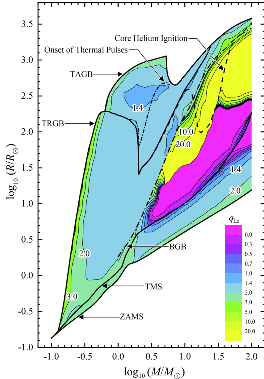
Figure 9. from The Thermal Equilibrium Mass-loss Model and Its Applications in Binary Evolution null 2020 APJS 249 9 doi:10.3847/1538-4365/ab98f6 https://dx.doi.org/10.3847/1538-4365/ab98f6 © 2020. The American Astronomical Society. All rights reserved.
