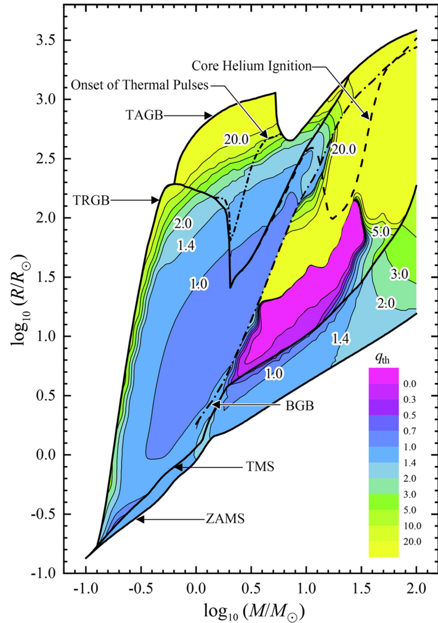
Figure 8. from The Thermal Equilibrium Mass-loss Model and Its Applications in Binary Evolution null 2020 APJS 249 9 doi:10.3847/1538-4365/ab98f6 https://dx.doi.org/10.3847/1538-4365/ab98f6 © 2020. The American Astronomical Society. All rights reserved.
