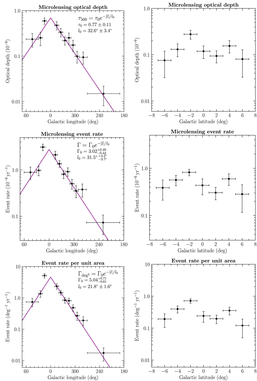
Figure 6. from Microlensing Optical Depth and Event Rate in the OGLE-IV Galactic Plane Fields null 2020 APJS 249 16 doi:10.3847/1538-4365/ab9366 https://dx.doi.org/10.3847/1538-4365/ab9366 © 2020. The American Astronomical Society. All rights reserved.
