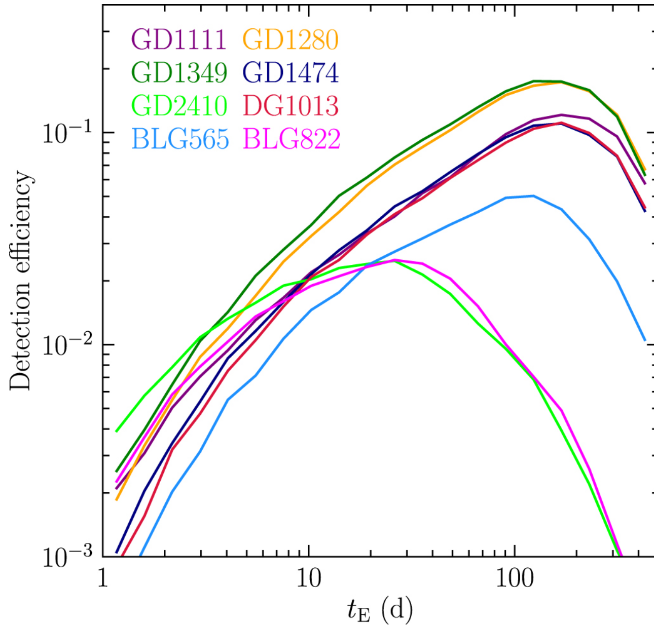
Figure 5. from Microlensing Optical Depth and Event Rate in the OGLE-IV Galactic Plane Fields null 2020 APJS 249 16 doi:10.3847/1538-4365/ab9366 https://dx.doi.org/10.3847/1538-4365/ab9366 © 2020. The American Astronomical Society. All rights reserved.
