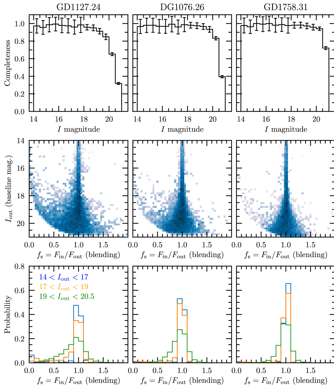
Figure 3. from Microlensing Optical Depth and Event Rate in the OGLE-IV Galactic Plane Fields null 2020 APJS 249 16 doi:10.3847/1538-4365/ab9366 https://dx.doi.org/10.3847/1538-4365/ab9366
