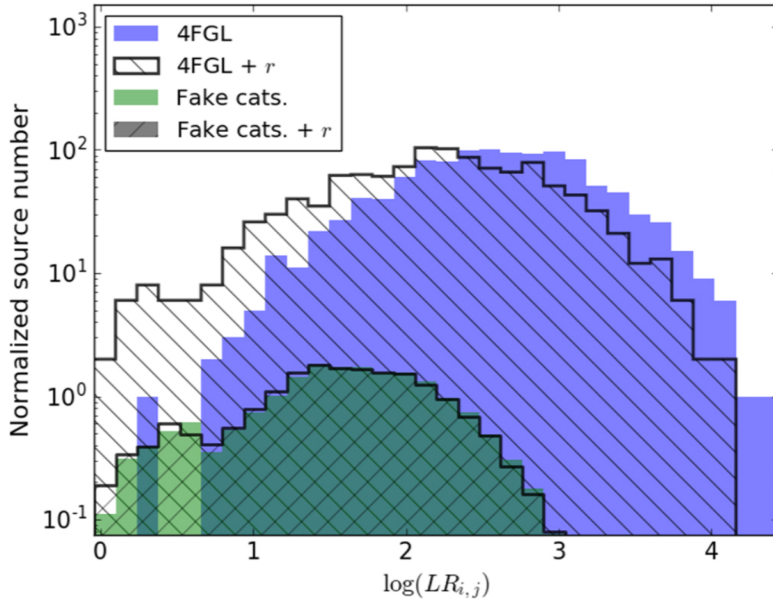
Figure 3. from On the Physical Association of Fermi-LAT Blazars with Their Low-energy Counterparts null 2020 APJS 248 23 doi:10.3847/1538-4365/ab8c4e https://dx.doi.org/10.3847/1538-4365/ab8c4e © 2020. The American Astronomical Society. All rights reserved.
