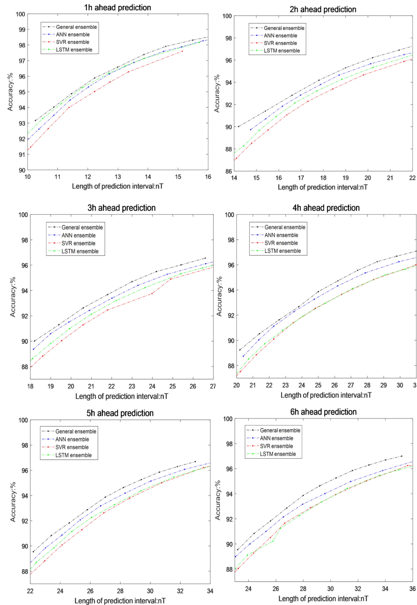
Figure 7. from Prediction of the Dst Index with Bagging Ensemble-learning Algorithm null 2020 APJS 248 14 doi:10.3847/1538-4365/ab880e https://dx.doi.org/10.3847/1538-4365/ab880e © 2020. The Author(s). Published by the American Astronomical Society.
