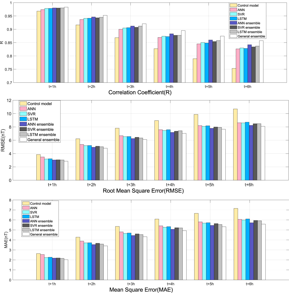
Figure 3. from Prediction of the Dst Index with Bagging Ensemble-learning Algorithm null 2020 APJS 248 14 doi:10.3847/1538-4365/ab880e https://dx.doi.org/10.3847/1538-4365/ab880e © 2020. The Author(s). Published by the American Astronomical Society.
