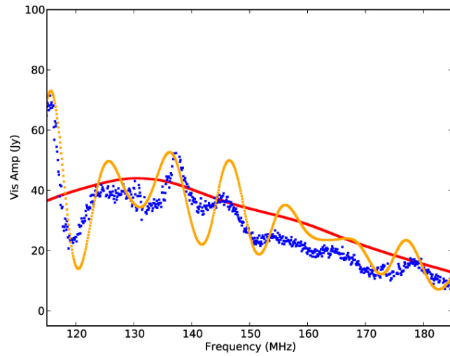
Figure 9. from Imaging and Modeling Data from the Hydrogen Epoch of Reionization Array null 2020 APJS 247 67 doi:10.3847/1538-4365/ab77b1 https://dx.doi.org/10.3847/1538-4365/ab77b1 © 2020. The American Astronomical Society. All rights reserved.
