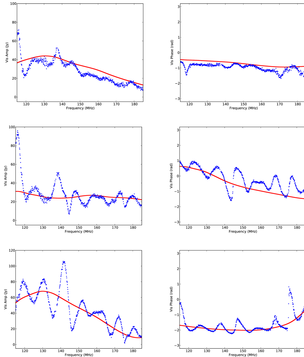
Figure 6. from Imaging and Modeling Data from the Hydrogen Epoch of Reionization Array null 2020 APJS 247 67 doi:10.3847/1538-4365/ab77b1 https://dx.doi.org/10.3847/1538-4365/ab77b1
