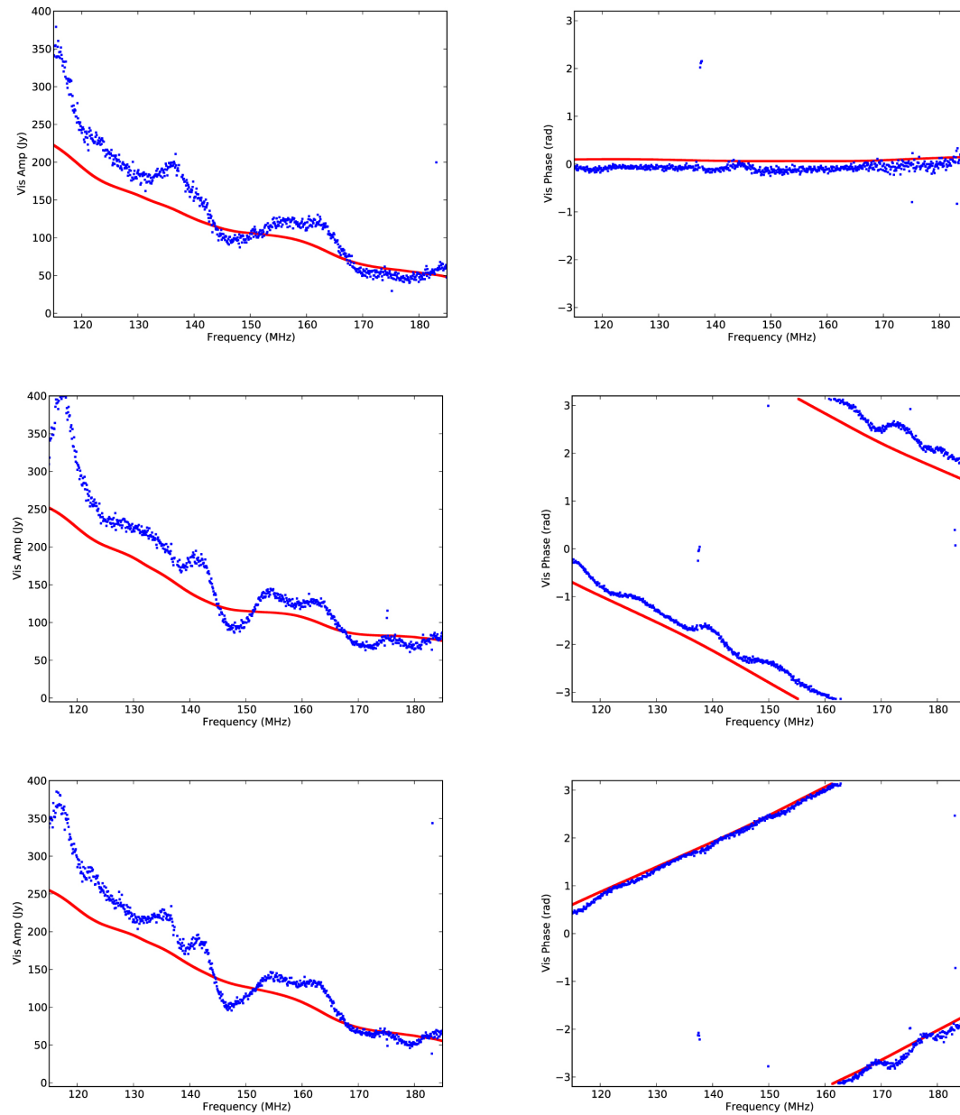
Figure 3. from Imaging and Modeling Data from the Hydrogen Epoch of Reionization Array null 2020 APJS 247 67 doi:10.3847/1538-4365/ab77b1 https://dx.doi.org/10.3847/1538-4365/ab77b1
