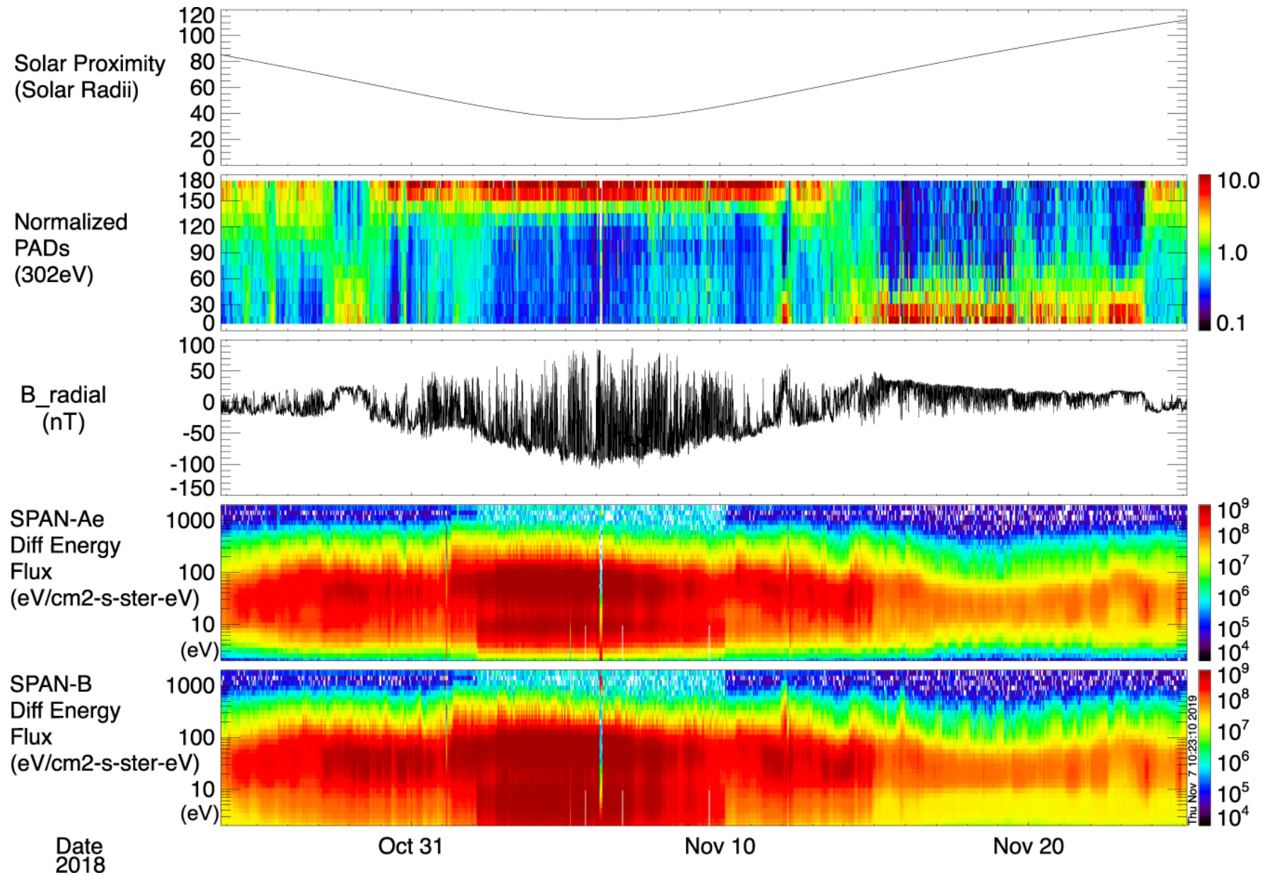
Figure 9. from The Solar Probe ANalyzers—Electrons on the Parker Solar Probe null 2020 APJS 246 74 doi:10.3847/1538-4365/ab7370 https://dx.doi.org/10.3847/1538-4365/ab7370 © 2020. The Author(s). Published by the American Astronomical Society.
