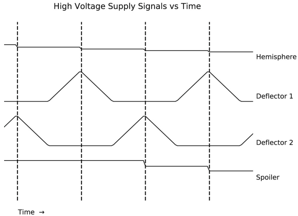
Figure 8. from The Solar Probe ANalyzers—Electrons on the Parker Solar Probe null 2020 APJS 246 74 doi:10.3847/1538-4365/ab7370 https://dx.doi.org/10.3847/1538-4365/ab7370 © 2020. The Author(s). Published by the American Astronomical Society.
