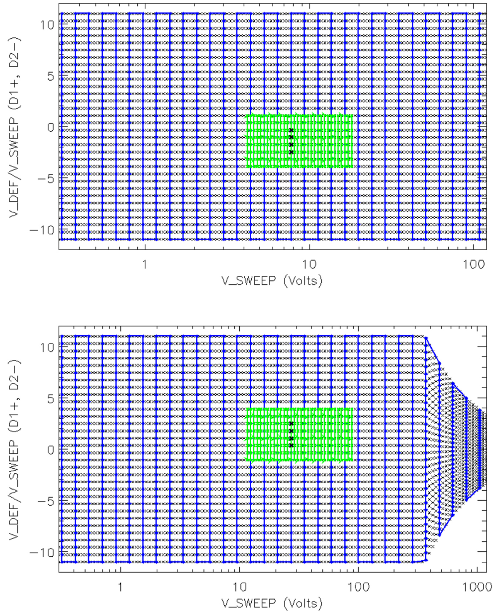
Figure 7. from The Solar Probe ANALYZERS—Electrons on the Parker Solar Probe null 2020 APJS 246 74 doi:10.3847/1538-4365/ab7370 https://dx.doi.org/10.3847/1538-4365/ab7370 © 2020. The Author(s). Published by the American Astronomical Society.
