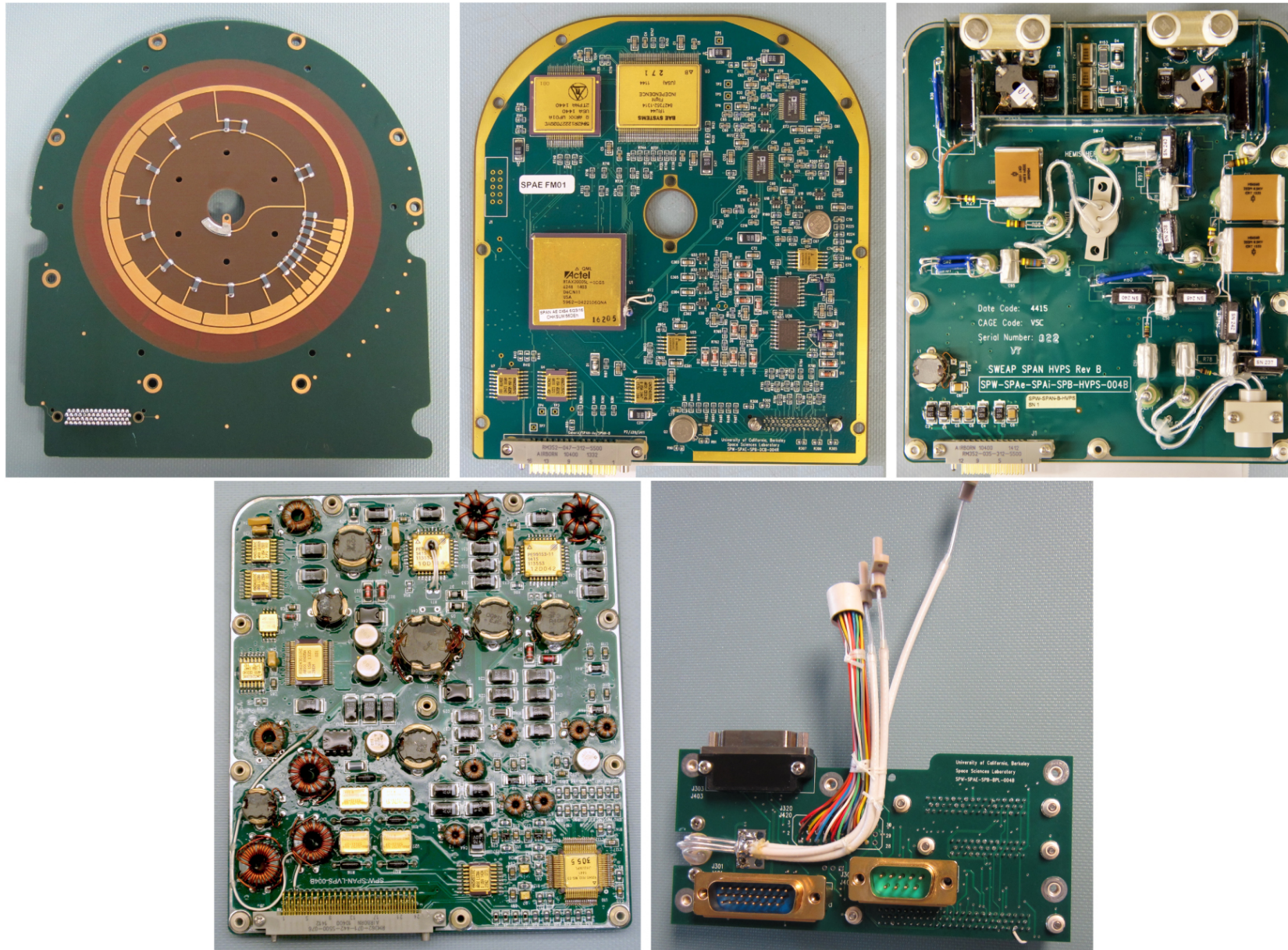
Figure 6. from The Solar Probe ANALYZERS—Electrons on the Parker Solar Probe null 2020 APJS 246 74 doi:10.3847/1538-4365/ab7370 https://dx.doi.org/10.3847/1538-4365/ab7370 © 2020. The Author(s). Published by the American Astronomical Society.
