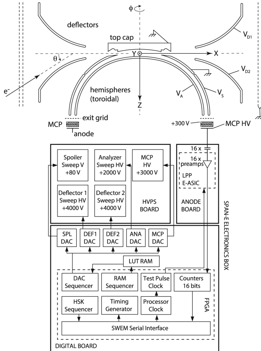
Figure 5. from The Solar Probe ANalyzers—Electrons on the Parker Solar Probe null 2020 APJS 246 74 doi:10.3847/1538-4365/ab7370 https://dx.doi.org/10.3847/1538-4365/ab7370 © 2020. The Author(s). Published by the American Astronomical Society.
