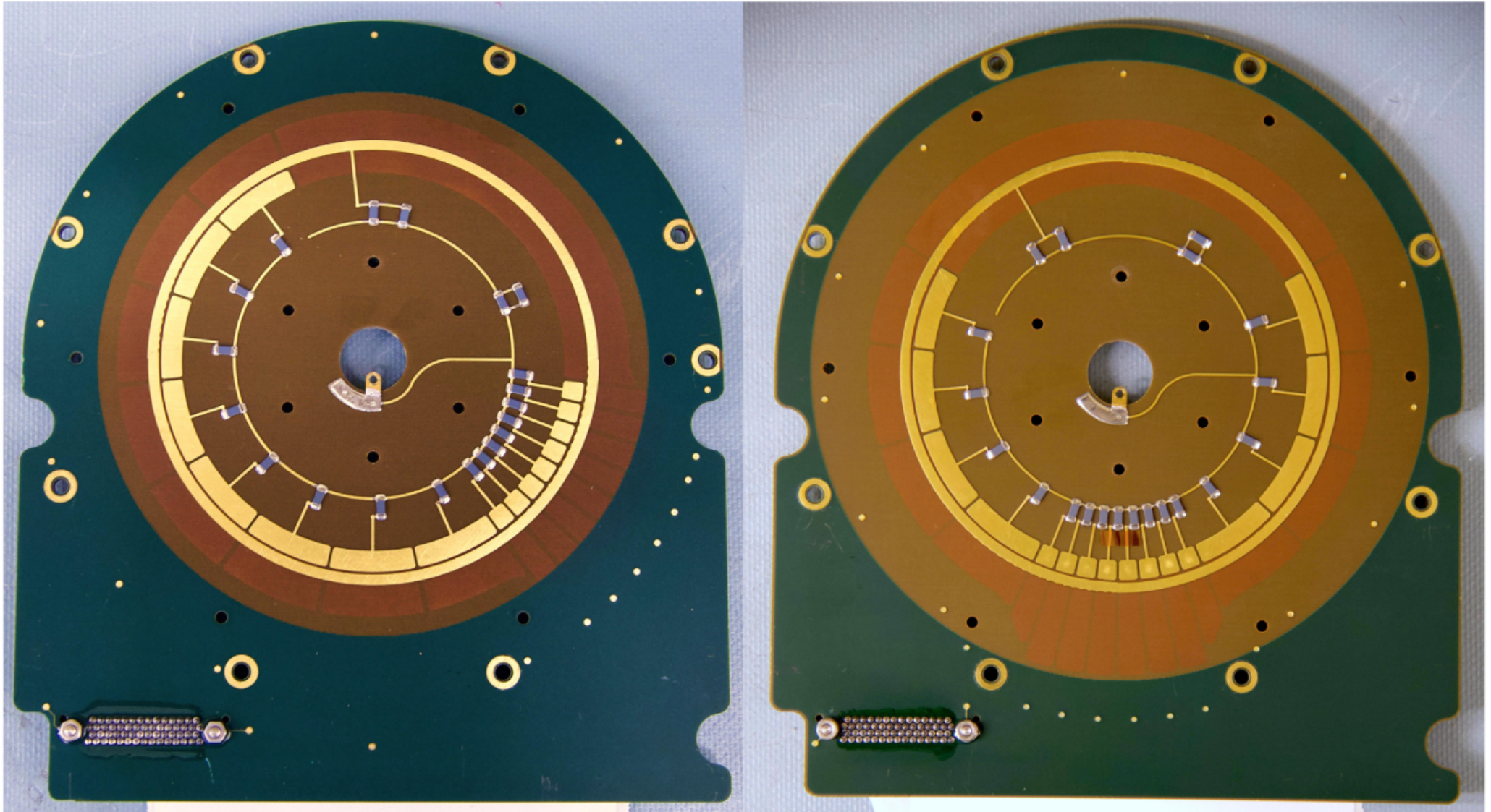
Figure 4. from The Solar Probe ANalyzers—Electrons on the Parker Solar Probe null 2020 APJS 246 74 doi:10.3847/1538-4365/ab7370 https://dx.doi.org/10.3847/1538-4365/ab7370 © 2020. The Author(s). Published by the American Astronomical Society.
