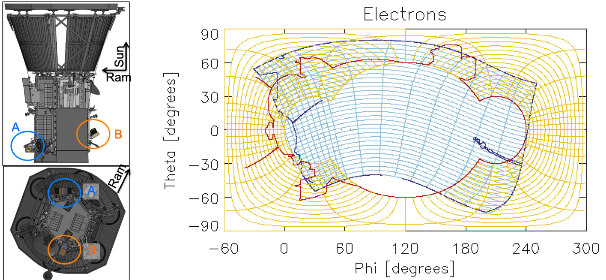
Figure 2. from The Solar Probe ANalyzers—Electrons on the Parker Solar Probe null 2020 APJS 246 74 doi:10.3847/1538-4365/ab7370 https://dx.doi.org/10.3847/1538-4365/ab7370 © 2020. The Author(s). Published by the American Astronomical Society.
