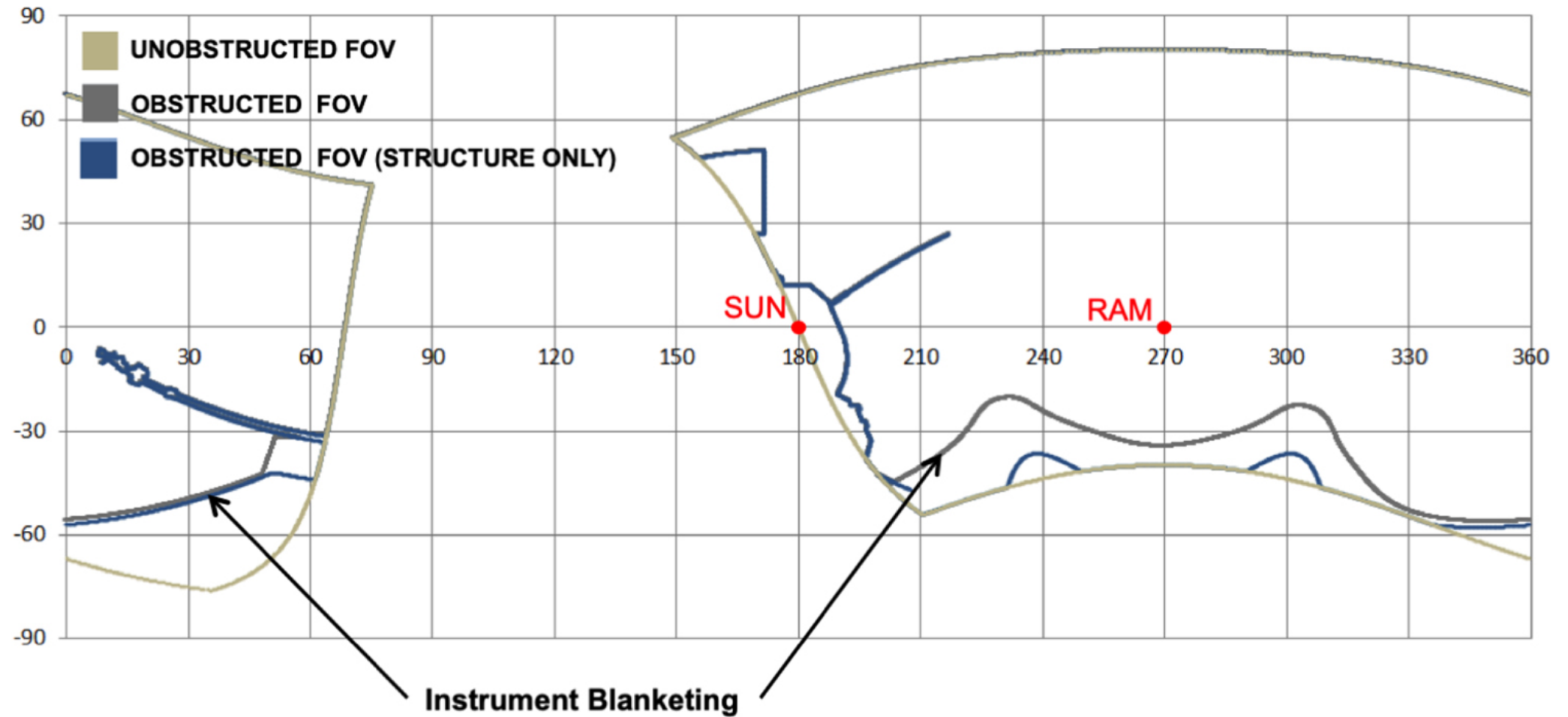
Figure 11. from The Solar Probe ANalyzers—Electrons on the Parker Solar Probe null 2020 APJS 246 74 doi:10.3847/1538-4365/ab7370 https://dx.doi.org/10.3847/1538-4365/ab7370 © 2020. The Author(s). Published by the American Astronomical Society.
